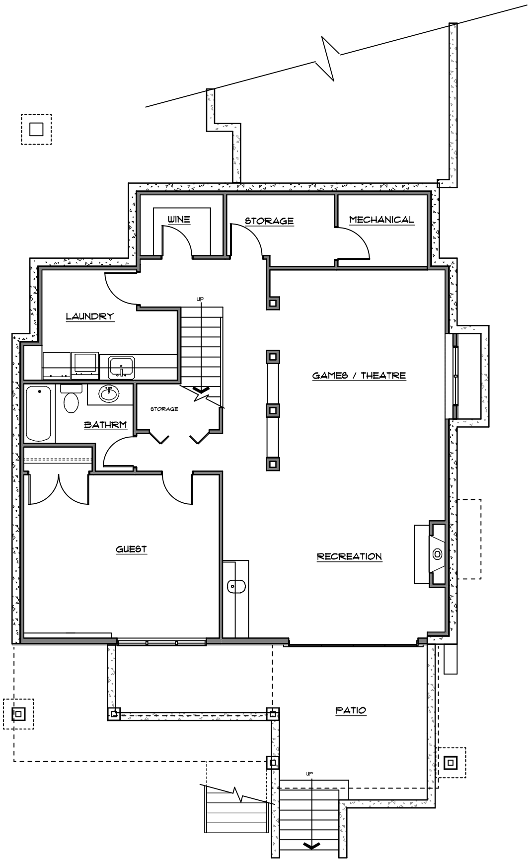
LOWER FLOOR PLAN
